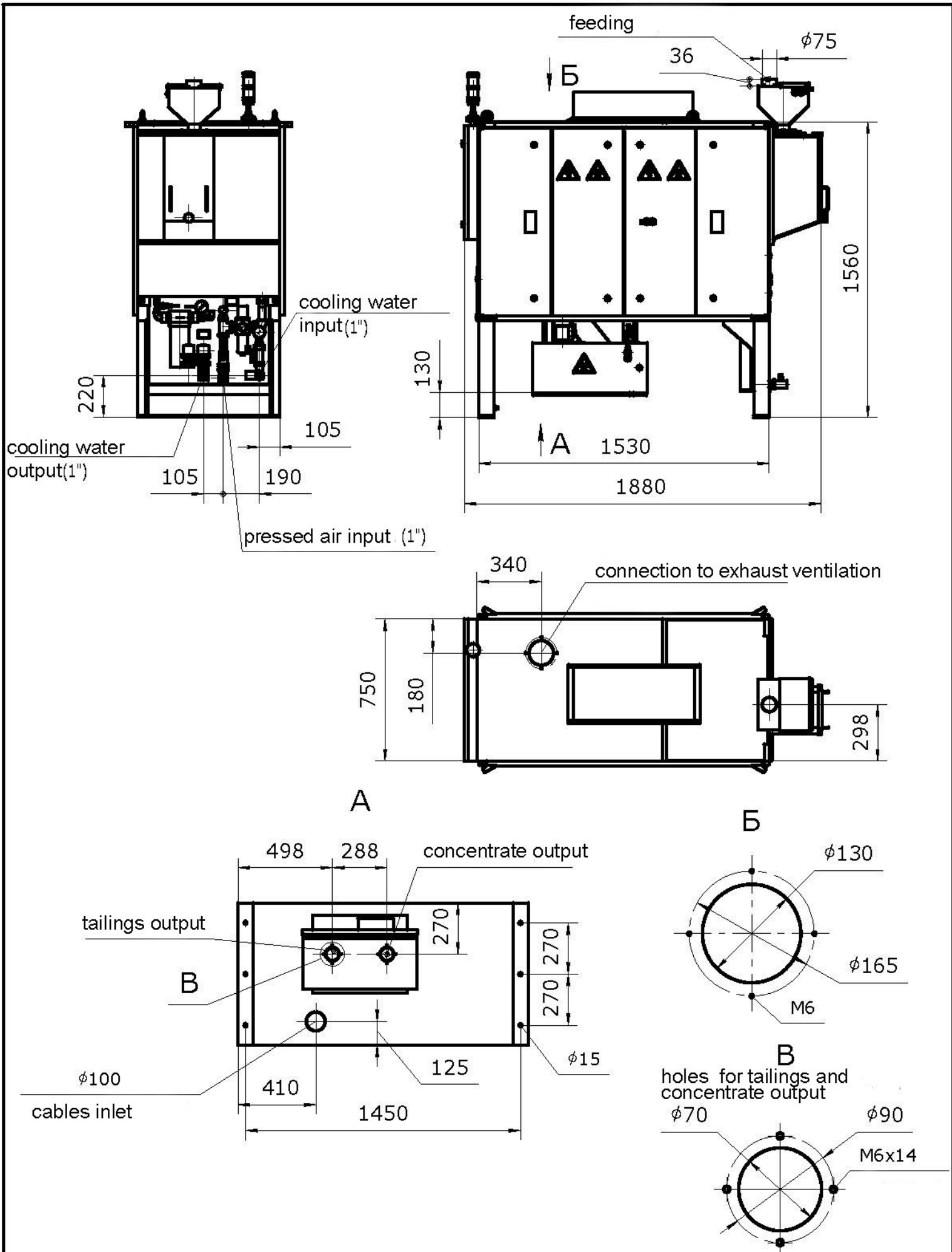
Sorting machine RGS-1M
