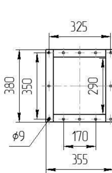
Sorting machine LS-OD-50-04-01
