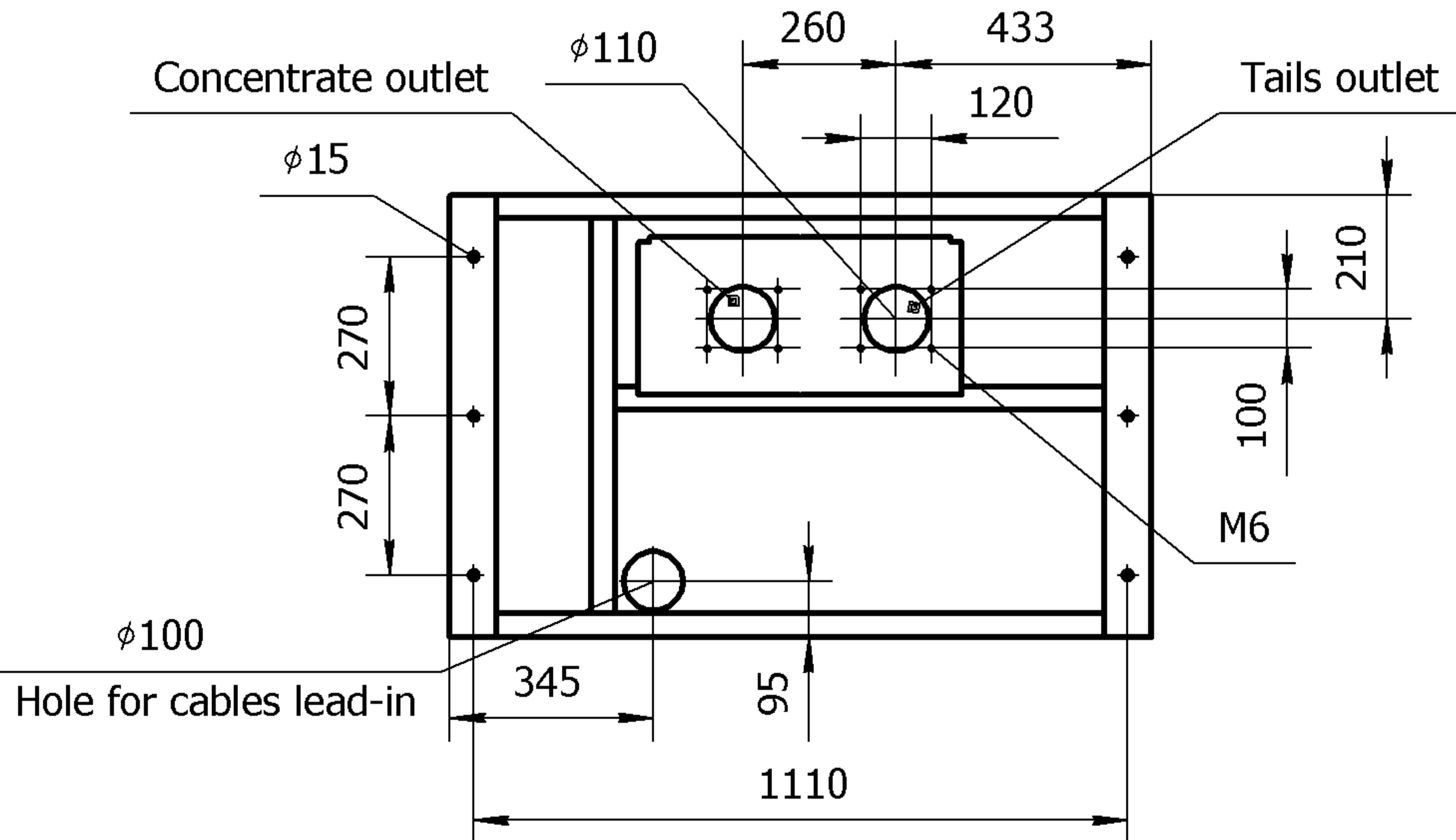
Sorting machine LS-D-4-03P
